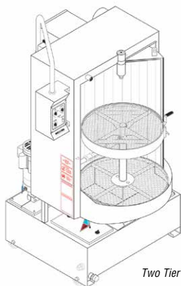
Filtration with Sump Sweep
